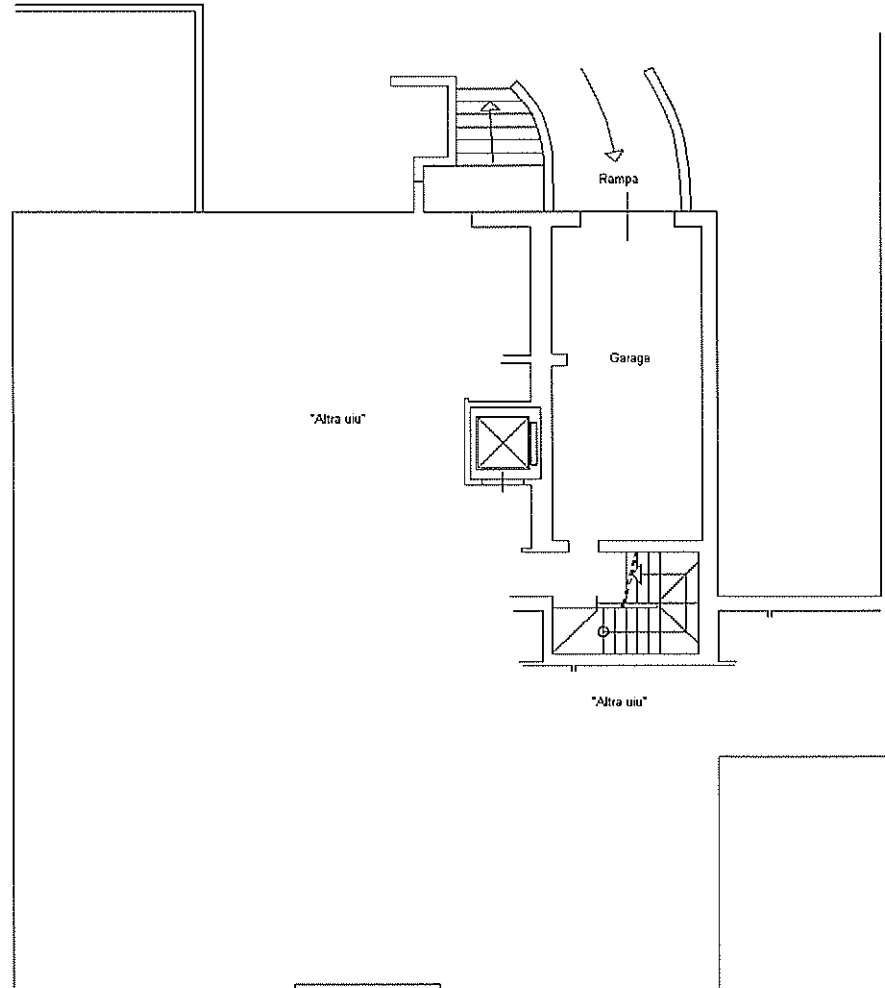
Piano Seminterrato 1 H= 3.00
